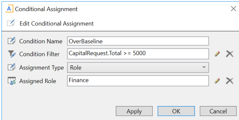
Example Conditional Assignment dialog using a role assignment
